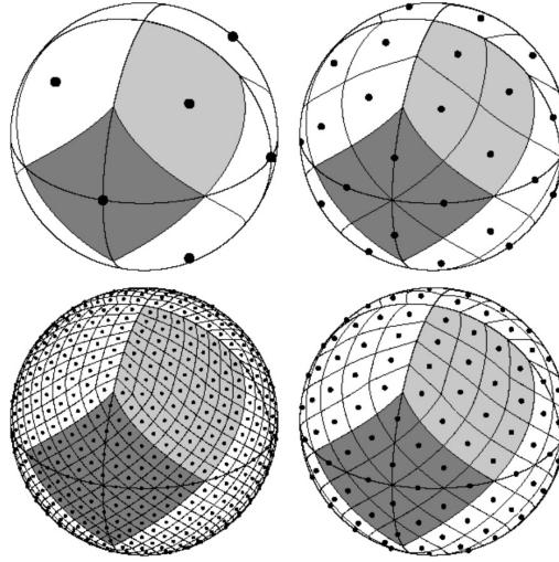
Figure 2.1: Visualization of HEALPix grid. Moving clockwise from the upper left panel the grid is hierarchically subdivided with the grid resolution parameter equal to N_{\text{side}} = 1, 2, 4, 8 , and the total number of pixels equal to N_{\text{pix}} = 12 \times N_{\text{side}}^2 = 12, 48, 192, 768
