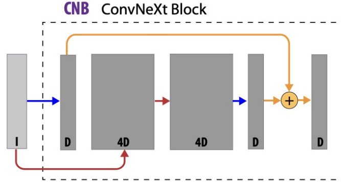
Figure 4.3: Representation of the ConvNeXt block [Karlbauer et al., 2023] . The orange arrows represent the Res-Net connection, blue arrows are the 1 \times 1 convolution, red arrows are 3 \times 3 convolutions, and D represent the depth or the number of channels.
